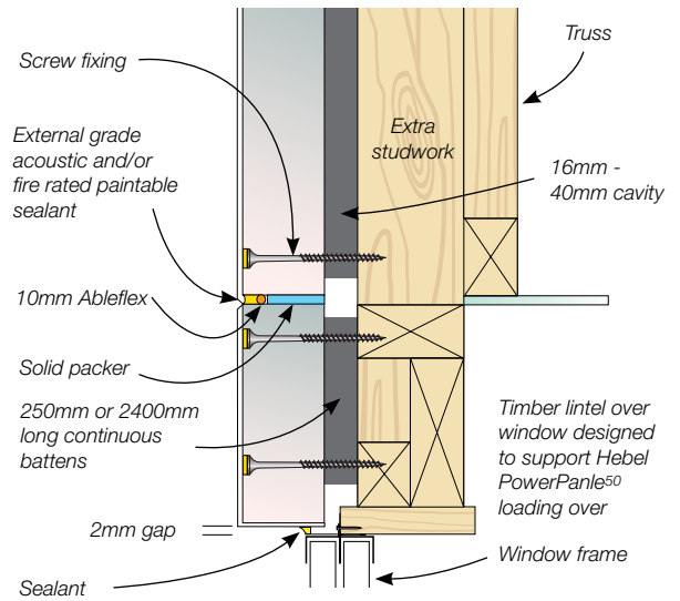
Figure 3.5.6.8 Gable end wall detail – lintel panel over window
