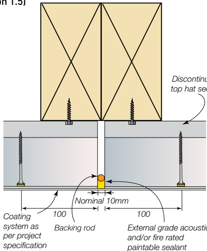
Figure 2.9.6.10 Typical vertical control joint with double studs (Achieves FRL 90/90/90 when installed as part of the wall system. See section 1.5)
