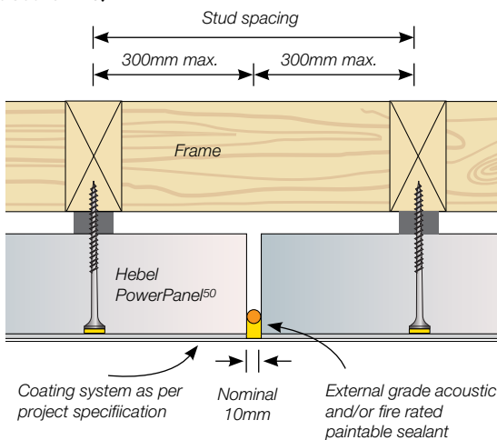
Figure 3.5.7.7 Typical vertical control joint [Achieves FRL 90/90/90 when installed as part of the wall system. See section 1.5]
