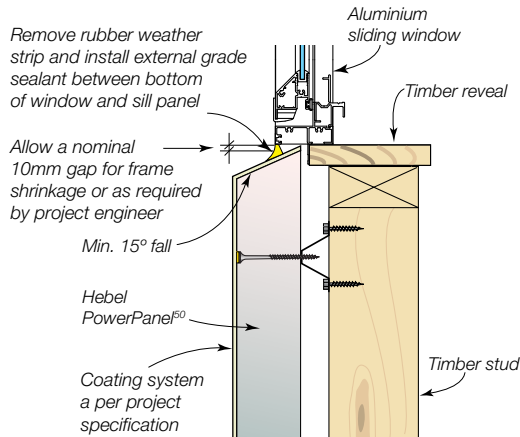
Figure 2.9.7.1 Typical window sill detail – aluminium window frame – Option 1
