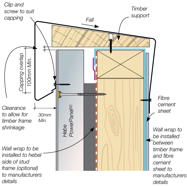
Figure 3.5.6.5 Parapet capping
