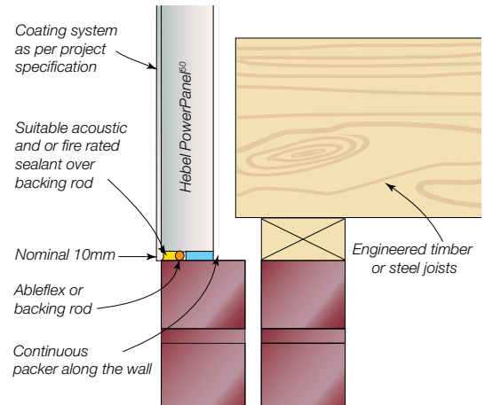
Figure 2.9.6.6 Horizontal control joint – Cavity brickwork to Hebel PowerPanel 50
