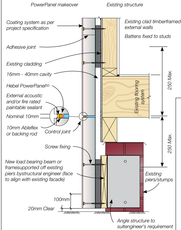
Figure 3.5.5.6 Base detail suspended floor – pier connection
