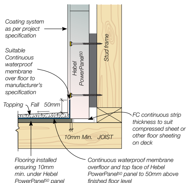
Figure 3.5.6.4 Balcony detail
